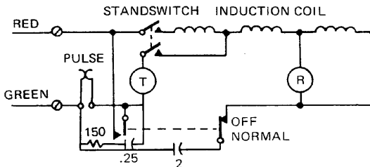
Figure 1.2. Ericofon Wiring Diagram Number 521031, for Manual and Dial Base Models without Ericotone (Models 52A and 52B).
