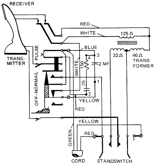
Schematic Diagram
