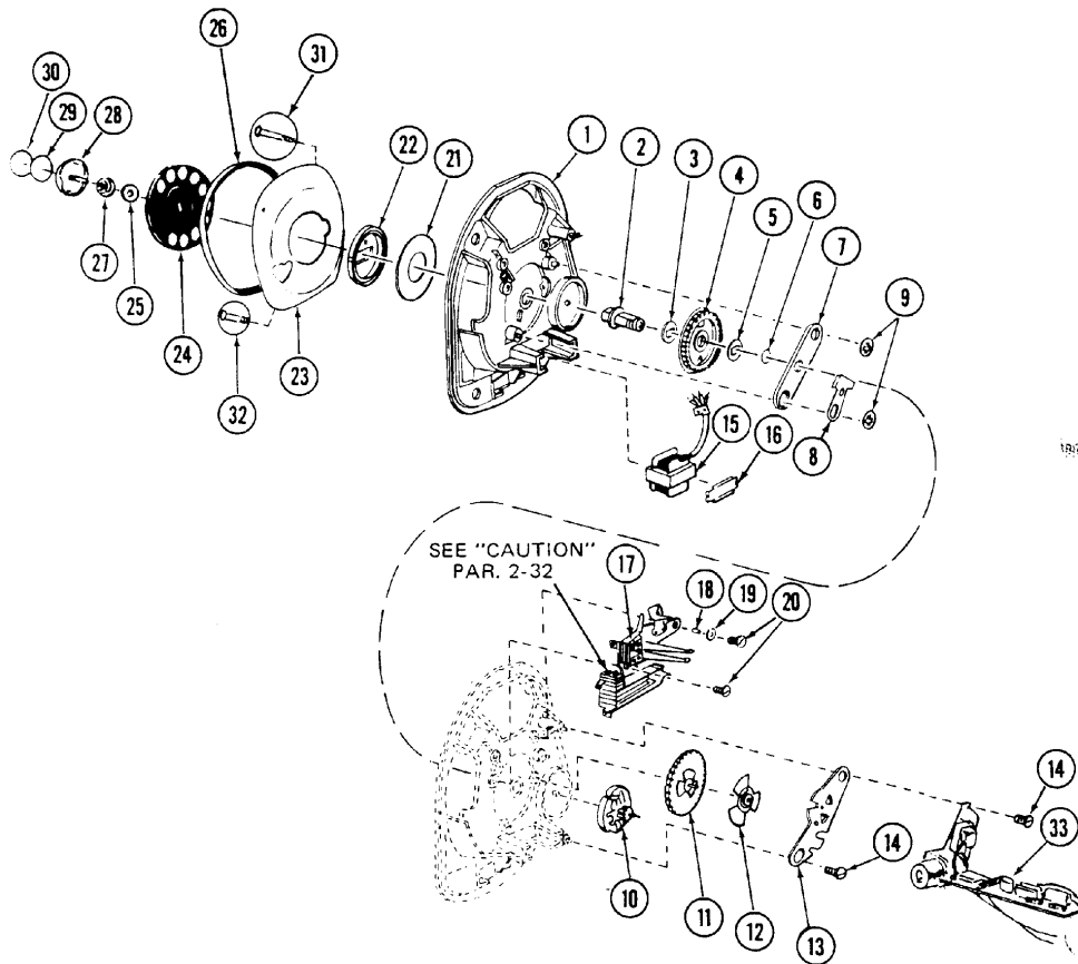
Figure 3.2. Base Assembly Part Number 520490
