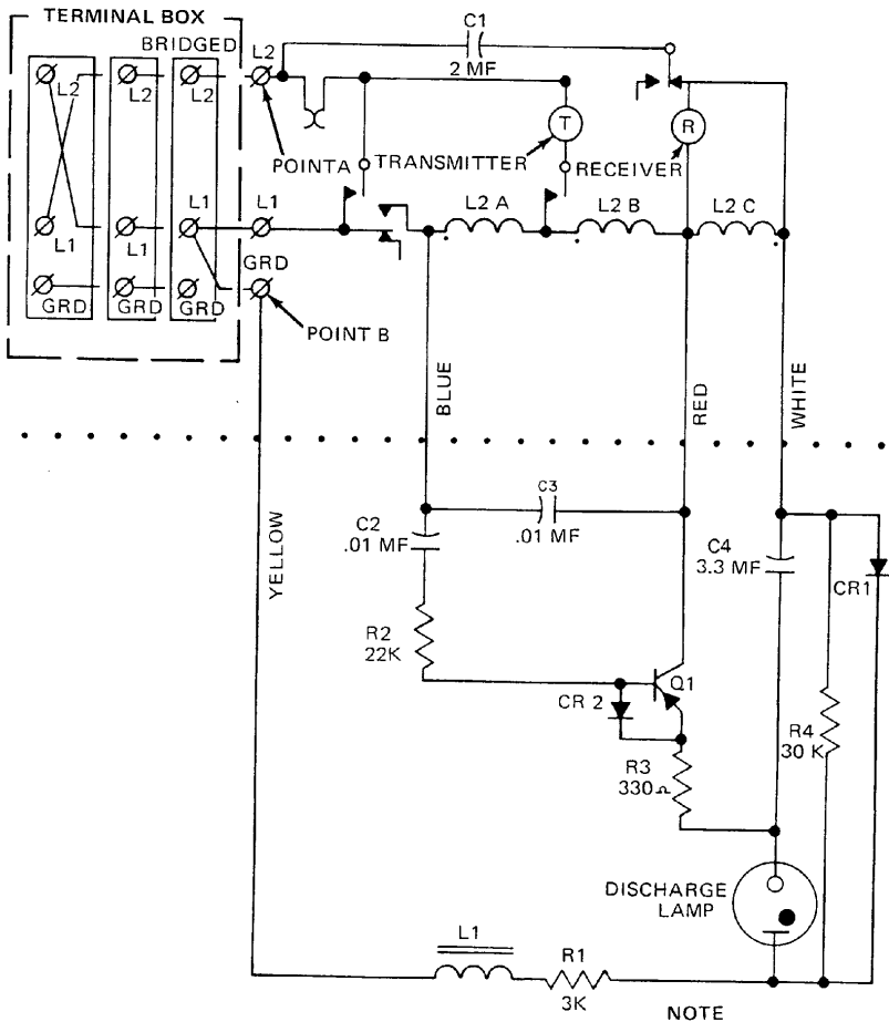
Figure 4.1. Schematic Diagram Showing the Electrical Relationship between the Ericofon and Ericotone Circuits
